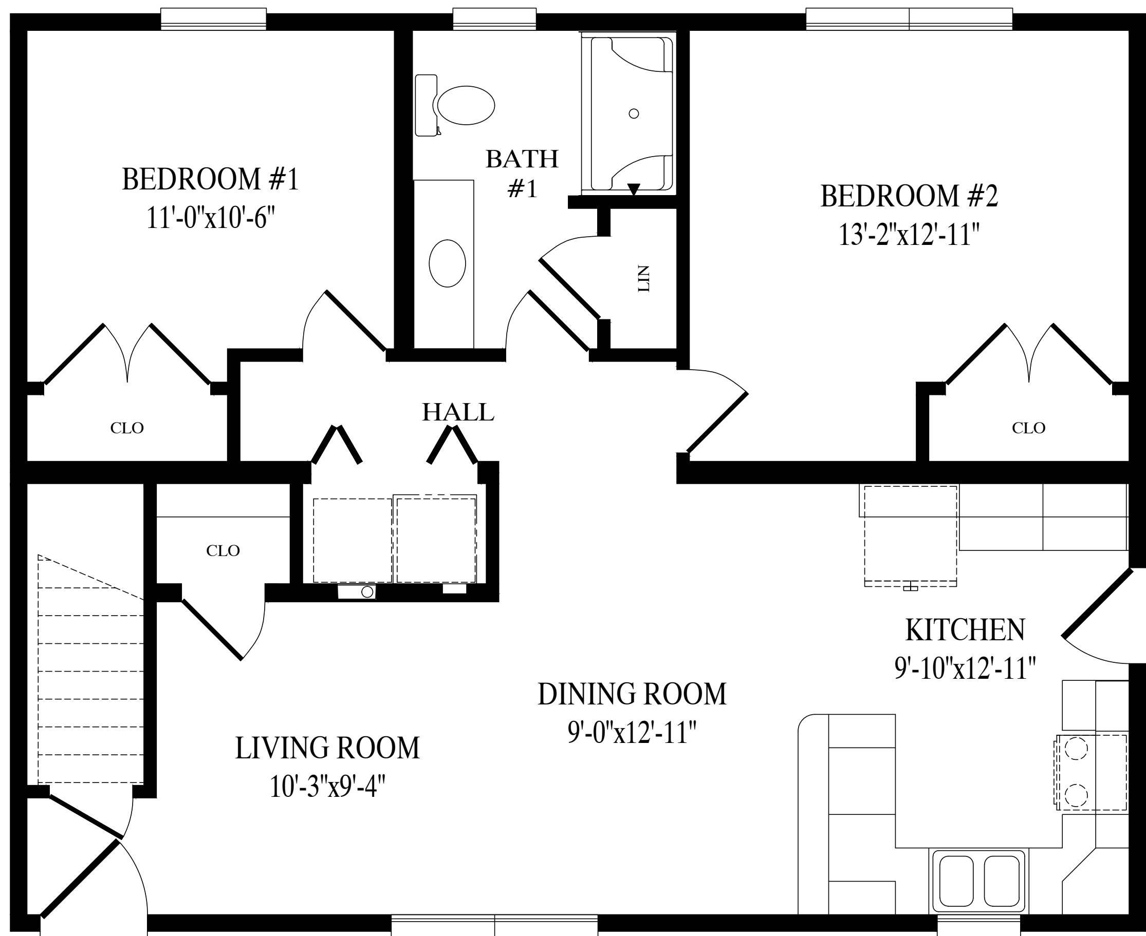
Exeter 27'-6" x 34' Ranch 935 sq. ft.
